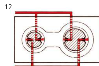
12. Measurement of hole distances of separated cylindrical bores with jet air plug gage measurement as per the differential measuring method.
