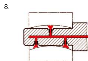
8. Straightness measurement of a cylindrical bore with special jet air plug gage.
